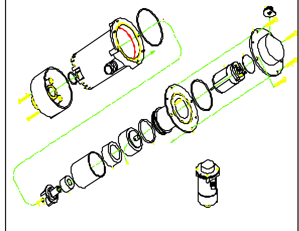
Exploded View—No Parts Kits Available
